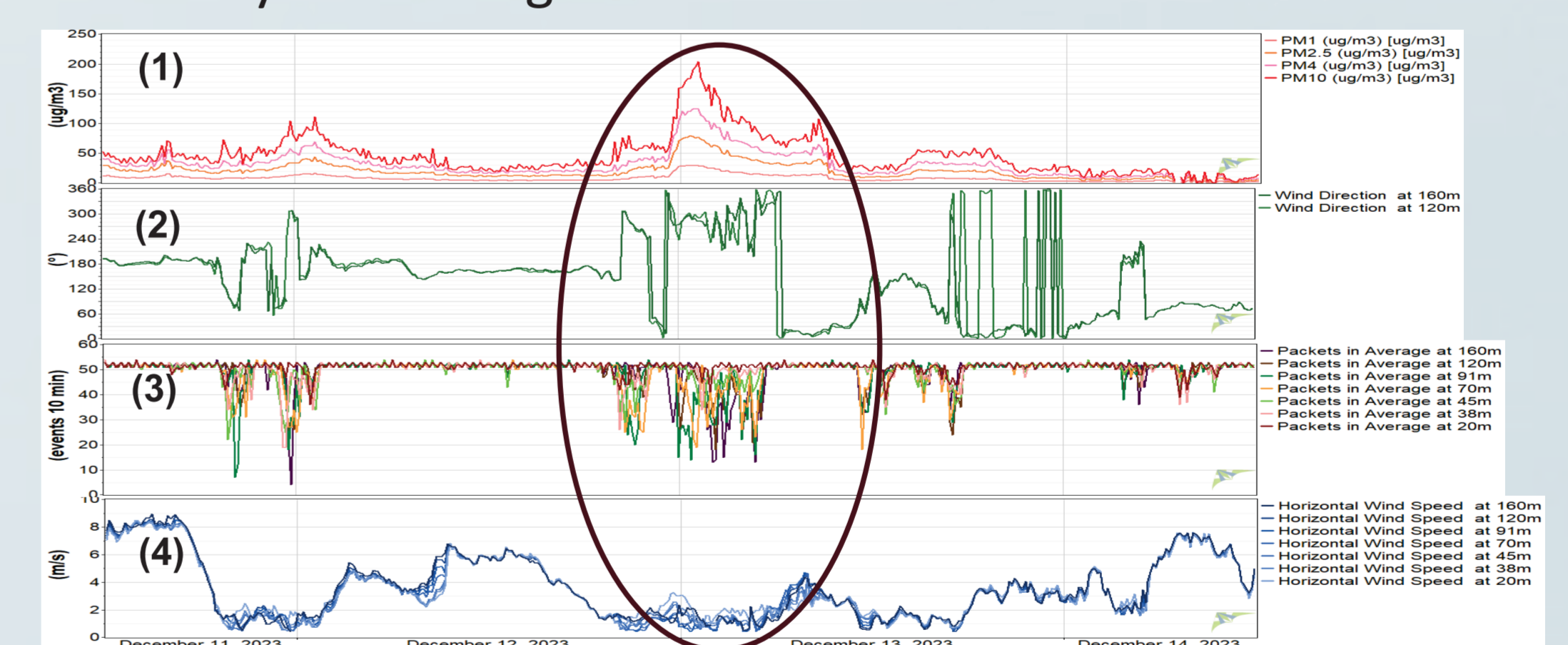
Figure 5. Data recorded in air quality station(1) and LIDAR, wind direction (2) availability (3) and wind speed (4).
