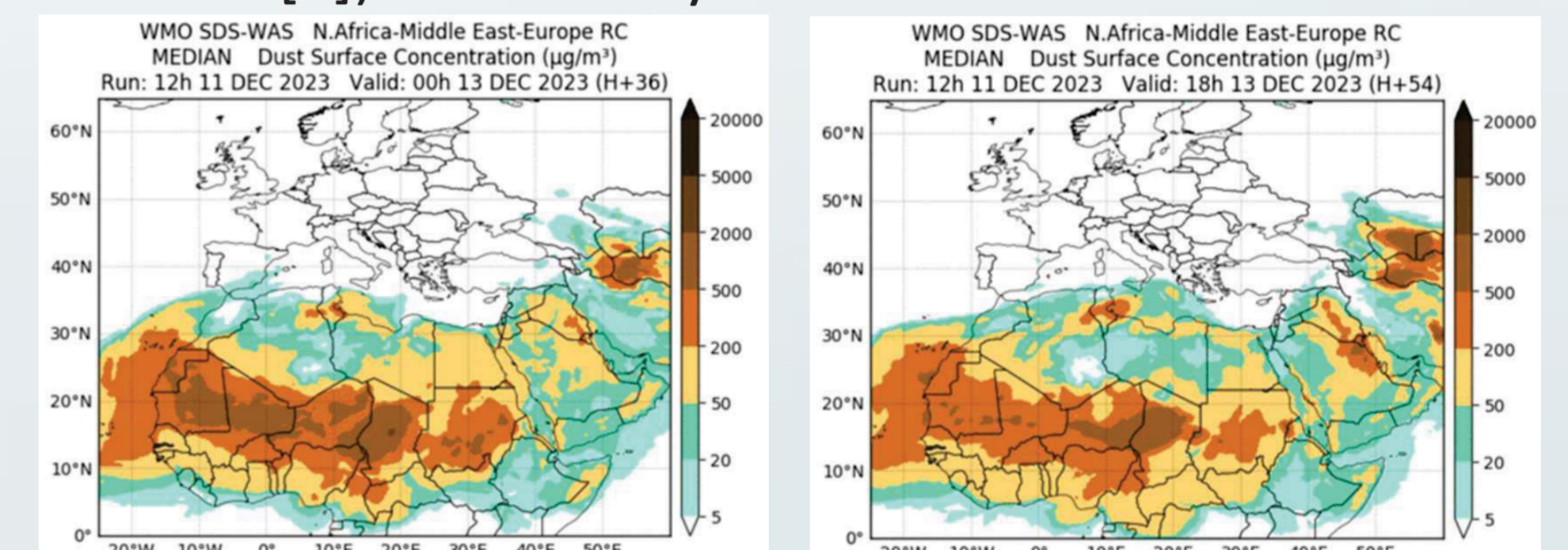
Figure 4. Results of MONARCH (median in µg/m 3 ) for 13 December 2023 at 00h UTC (left) and 18h UTC (right). Sand and Dust Storm Warning Advisory and Assessment System Regional Center for Northern Africa, Middle East and Europe (SDS-WAS NAMEE RC) [4], jointly managed by the State Meteorological Agency [5] and Barcelona Supercomputing Center[6].
